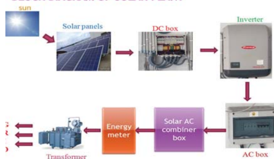
BLOCK DIAGRAM OF SOLAR PLANT
